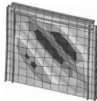
Fig 1: Formation of tension field
