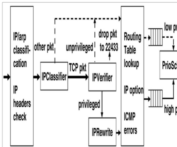
Fig 3.1. WRAPS elements on a Click packet forwarding path
