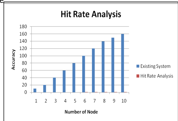
Fig 4.1HitRate-Performances Analysis
