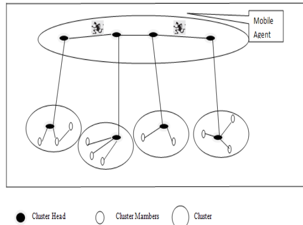
Fig 5: Structure of clustered of WSN with a mobile Agent
