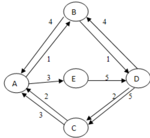
Figure 4 Routers Path
