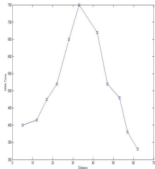
Fig. 10. HNA vs. the distance between cluster heads
