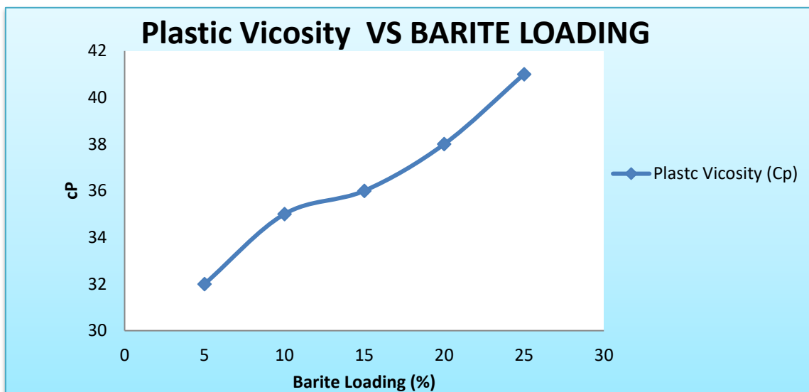
Fig. 8: Graph of PV (cP) against Barite Loading (%).
