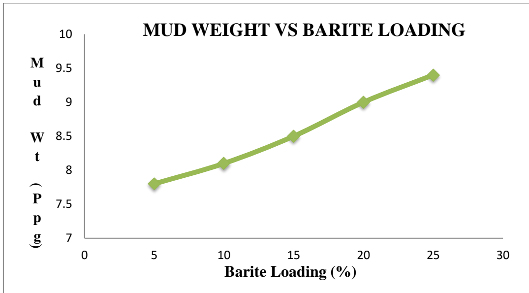
Fig 6: Graph of Mud Weight (ppg) against Barite Loading (%)
