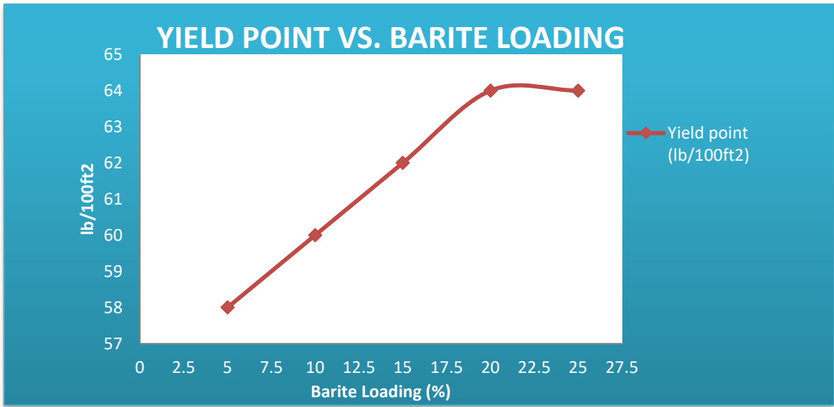
Fig. 9: Graph of YP (lb/100ft 2 ) against Barite Loading (%).
