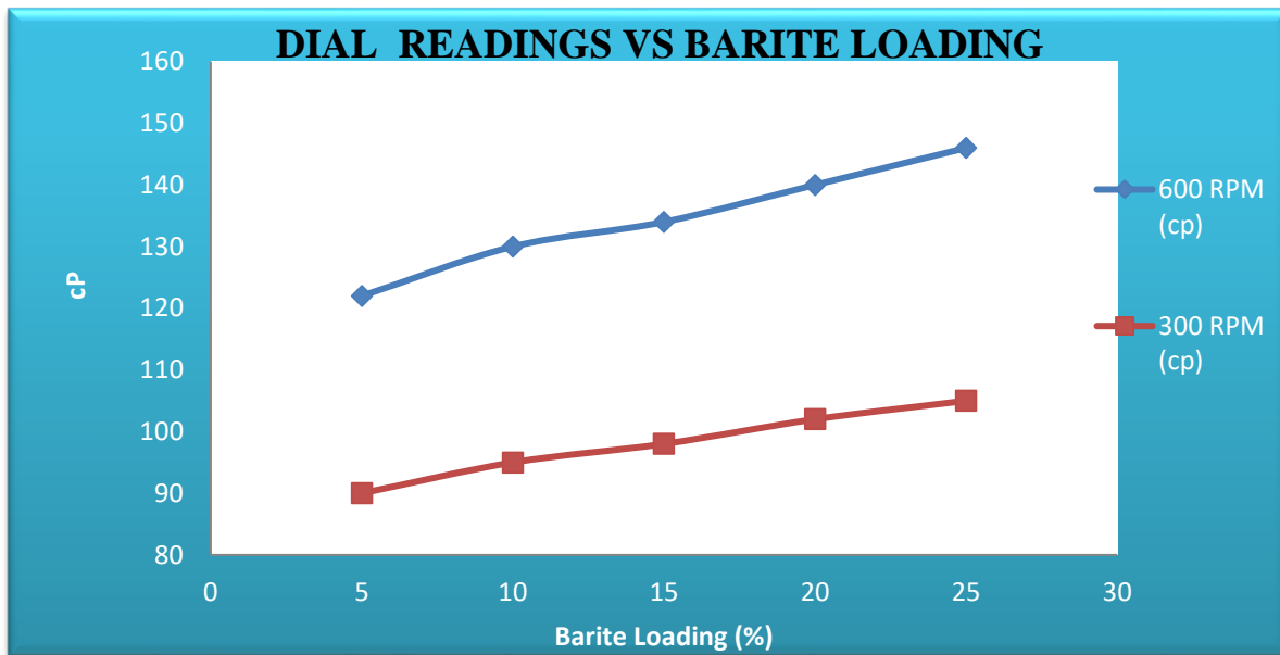
Fig7: Graph of 600RPM (cP) and 300RPM (cP) against Barite Loading (%)
