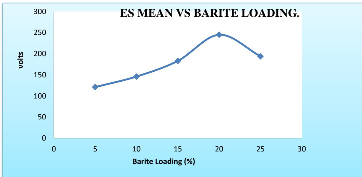
Fig. 11: Graph of Electrical Stability (Volts) against Barite Loading (%).
