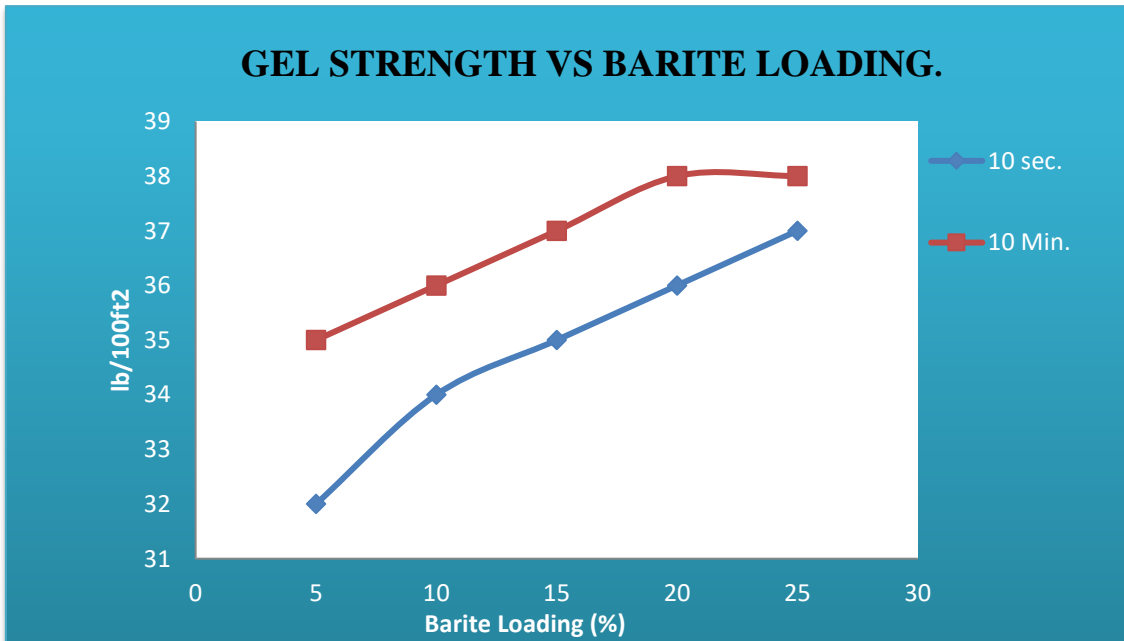
Fig.10: Graph of Gel Strength at 10sec (lb/100ft 2 ) and 10min (lb/100 2 ) against Barite Loading (%).
