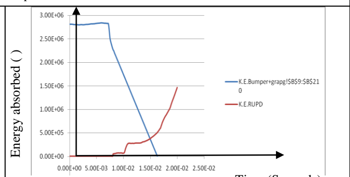
Fig 2.4 Simulation & energy absorption in car bumper and RUPD with thickness 4.50 mm
