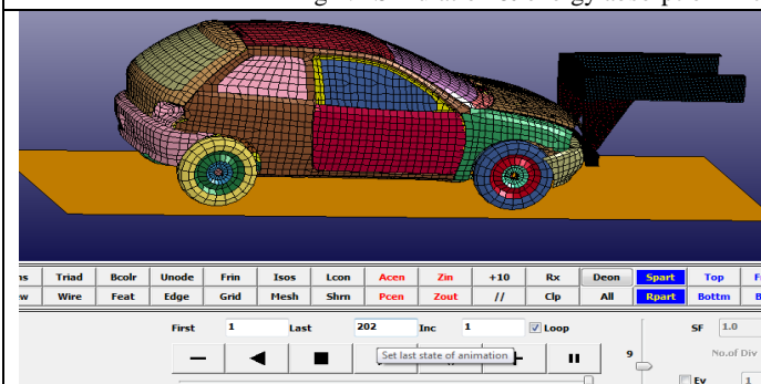
Fig 2.5 Simulation & energy absorption in car bumper and RUPD with thickness 5.00 mm
