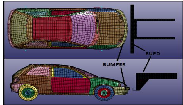
Fig. 1.1 Car Bumper and RUPD
