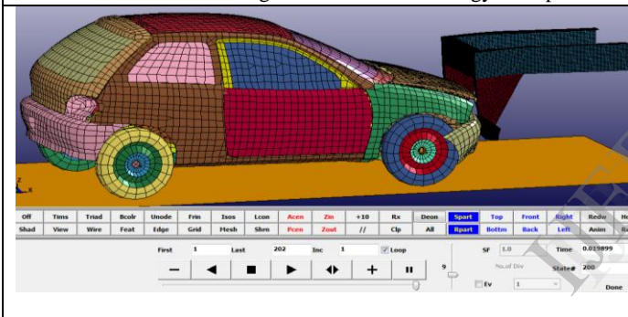
Fig 2.3 Simulation & energy absorption in car bumper and RUPD with thickness 4.00 mm
