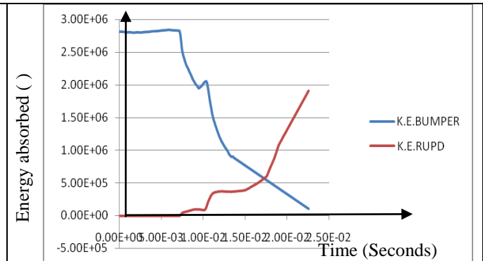
Fig 2.1 Simulation & energy absorption in car bumper and RUPD with thickness 3.00 mm
