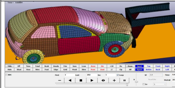
Fig 2.2 Simulation & energy absorption in car bumper and RUPD with thickness 3.50 mm
