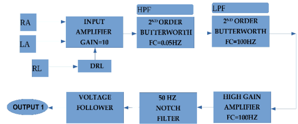
Fig 4.1: Proposed block diagram-ECG
