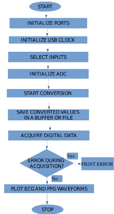
Fig 5.1: Program flowchart
