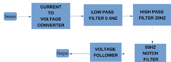
Fig 4.2: Proposed block diagram-PPG
