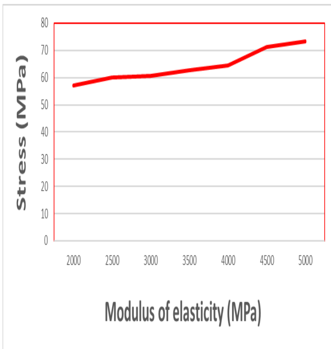
Fig. 6. Graph of elastic modulus v/s stress of asphalt layer
