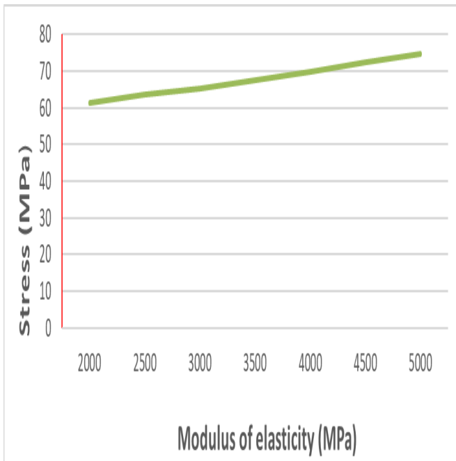
Fig. 2. Graph of elastic modulus v/s stress of asphalt layer
