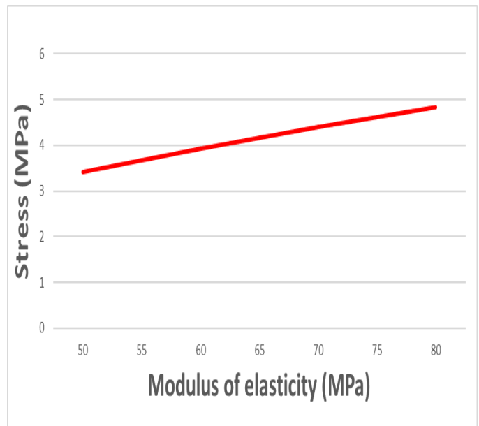
Fig. 7. Graph of elastic modulus v/s stress of base layer
