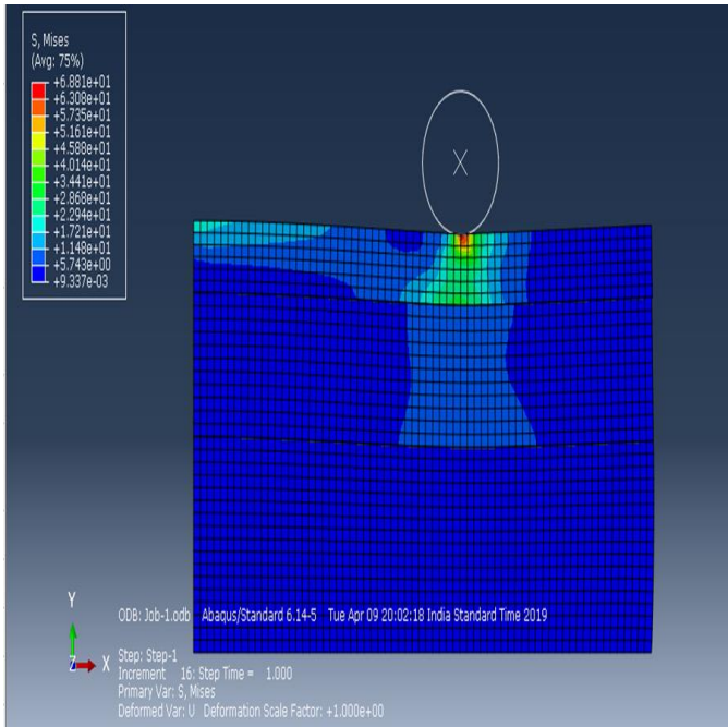
Fig. 1. Stresses at different layers of pavement without geogrid
