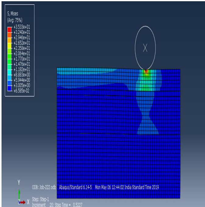
Fig. 5. Stresses at different layers of pavement with geogrid
