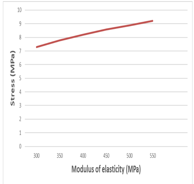
Fig. 3. Graph of elastic modulus v/s stress of base layer
