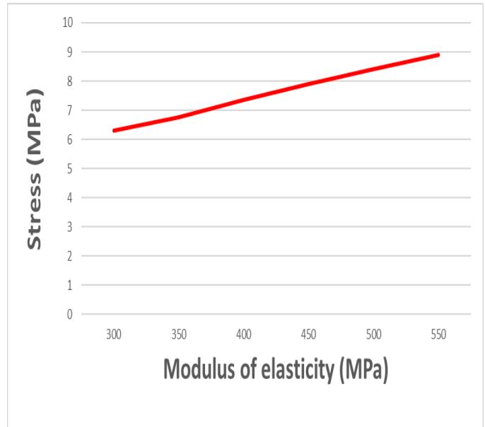
Fig. 7. Graph of elastic modulus v/s stress of base layer
