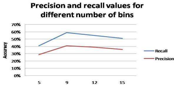
Fig. 14. Effect of number of bins change using HOG method. The block size is constant 5.
