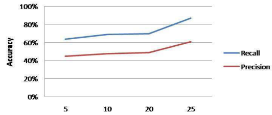
Fig. 11. Effect of block size change using EHD method. The threshold is constant 2.
