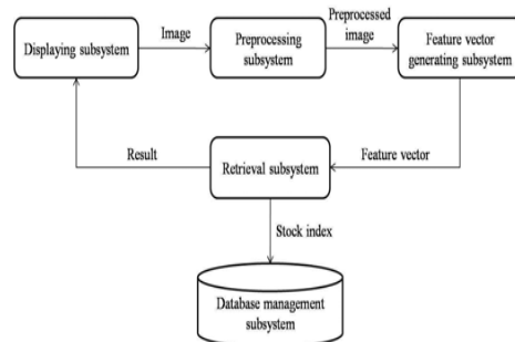
Fig. 1. The global structure of the system.
