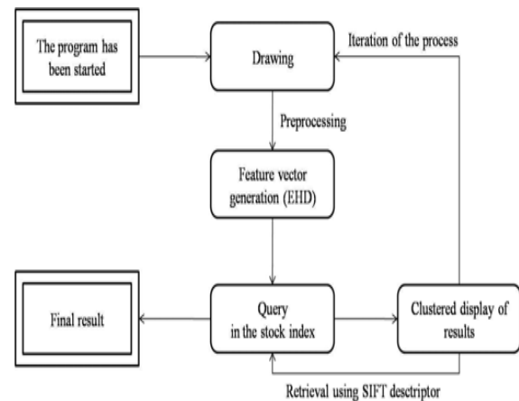
Fig. 2. The data flow model of the system from the user's point of view.
