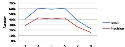
Precision and recall values for different blocksize values
