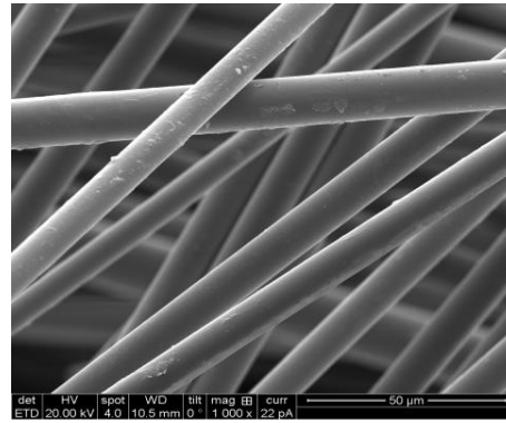
Fig. 1 (f) SEM Micrographs of coated basalt fibers
