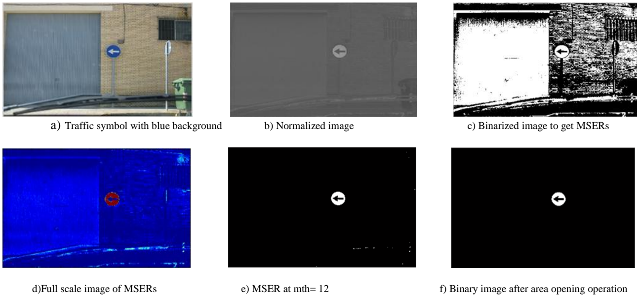
Fig. 3. Fig (a)-(f) detection of traffic sign image as MSERs.
