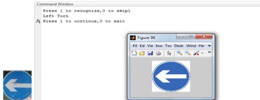
(e) Extracted image (f) Recognized traffic sign
