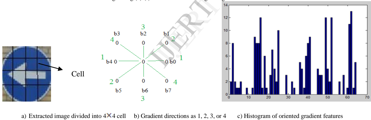
Fig. 4. Fig (a)-(c) HOG feature extraction.
