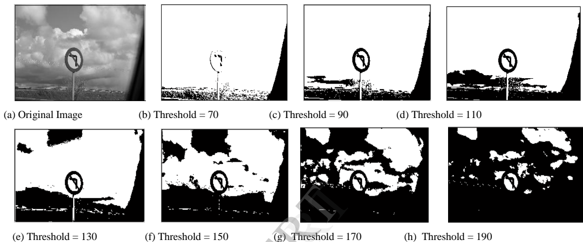
Fig. 2. Fig(a)-(i) Connected components at several thresholds for original image.
