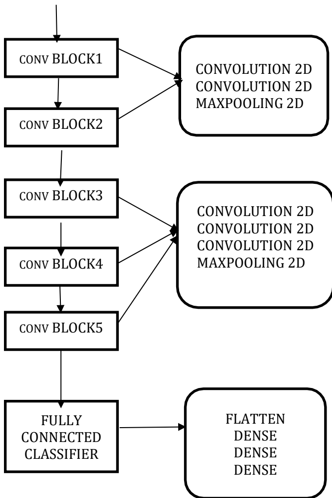
Fig.3.a.Architecture of VGG16
