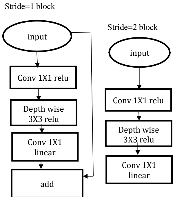
Fig.4.a.convolution of MobileNetV2
