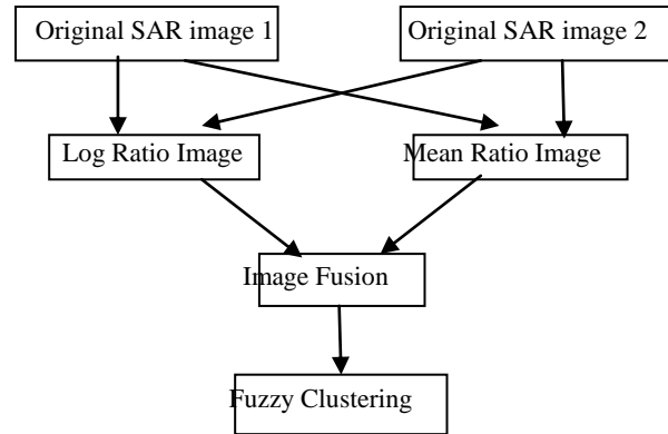
Fig. 1. Flowchart of the proposed change detection approach.
