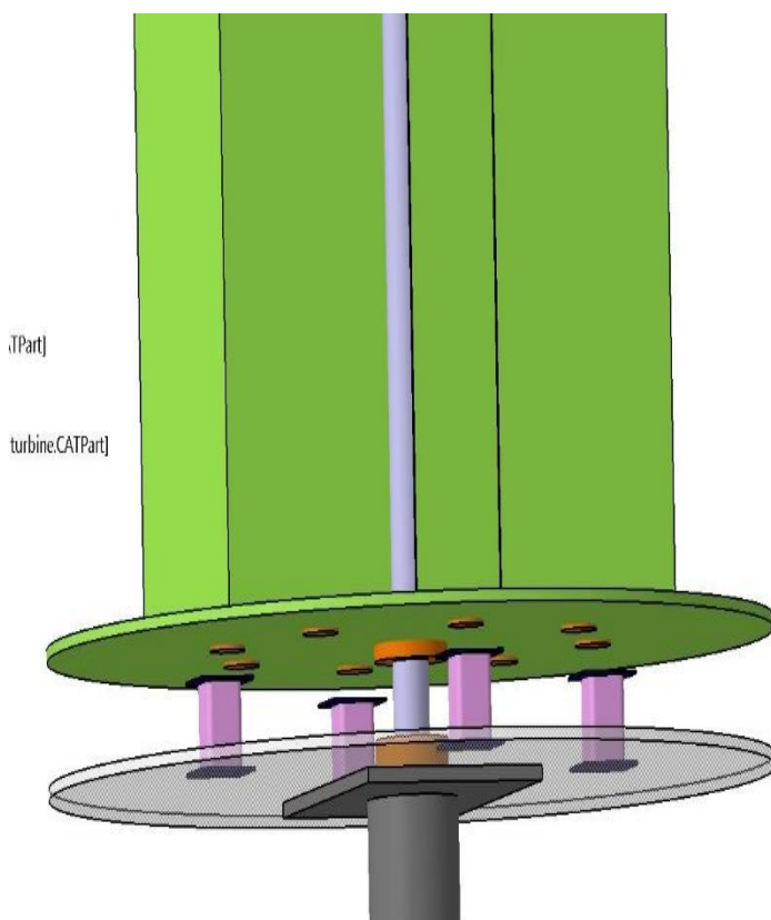
Fig.6 Stand of Rotor
