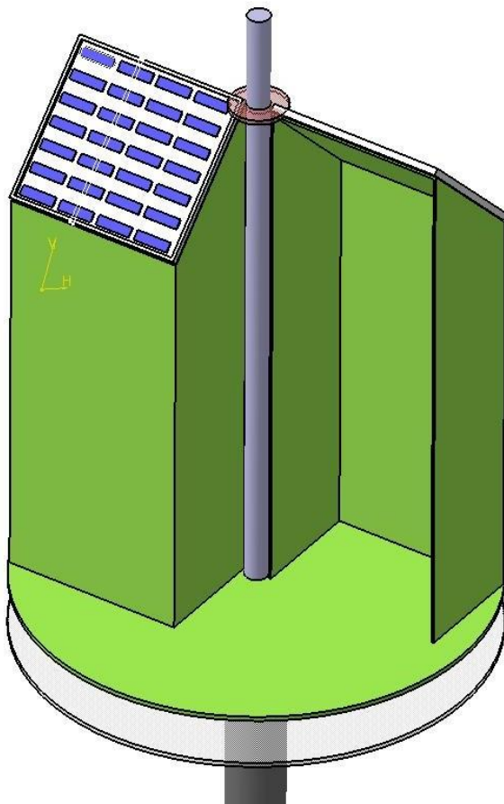
Fig.5 Rotated view of S-type rotor
