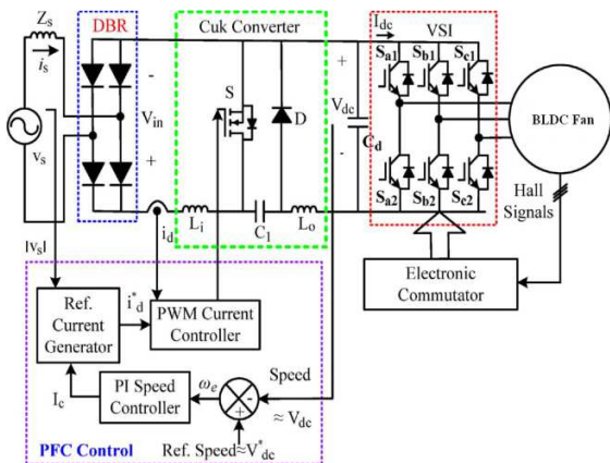
Fig. 1. Control scheme of the proposed Cuk PFC converter – fed VSI- based PMBLDCM
