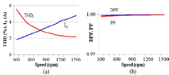
Fig. 4. PQ indices of proposed drive under speed control at rated torque and 220 V ac input. (a) Variation of I_s and its THD. (b) Variation of DPF and PF
