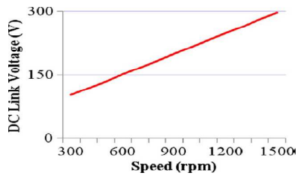
Fig.3. Variation of dc link voltage with speed for proposed PFC drive at rated torque and 220 V ac input
