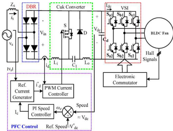
Fig. 1. Control scheme of the proposed Cuk PFC converter – fed VSI- based PMBLDCM
