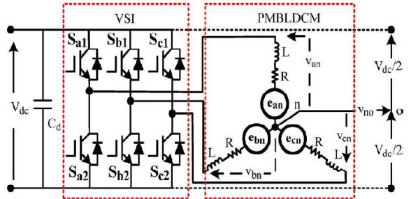
Fig.2. Equivalent circuit of a VSI-fed PMBLDCMD
