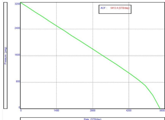
Figure 2.0: IPR curve of a low productivity index well
