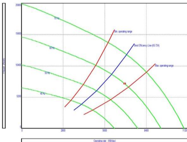
Figure 4: ESP Design plot for low productivity index well
