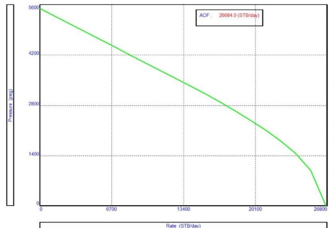
Figure 4: IPR Curve for high productivity index well
