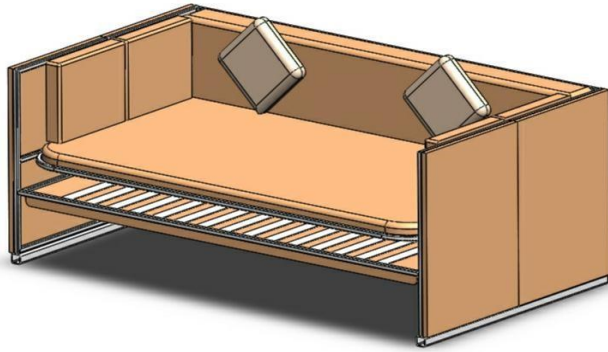
Figure 3: Design of BUNK BED WITH LEISURE SOFA (fully finished product) SOFA STAGE
