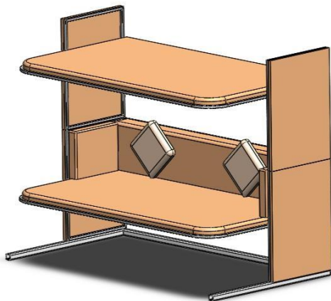
Figure 4: Design of BUNK BED with LEISURE SOFA (fully finished product) BUNK BED STAGE.
