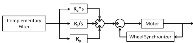
Fig. 9. Block diagram of balancing robot
