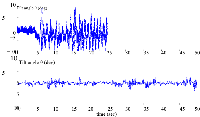
Fig. 12. Experimentally obtained history of tilt angle: PID controller (top), PI-PD controller (bottom).
