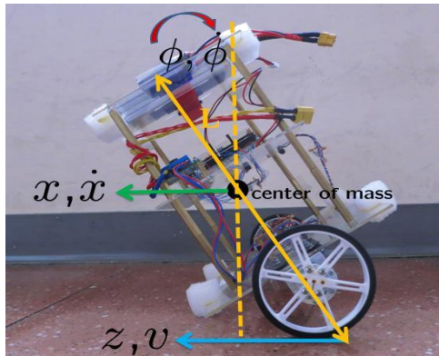
Fig. 8. Definition of motion variables
