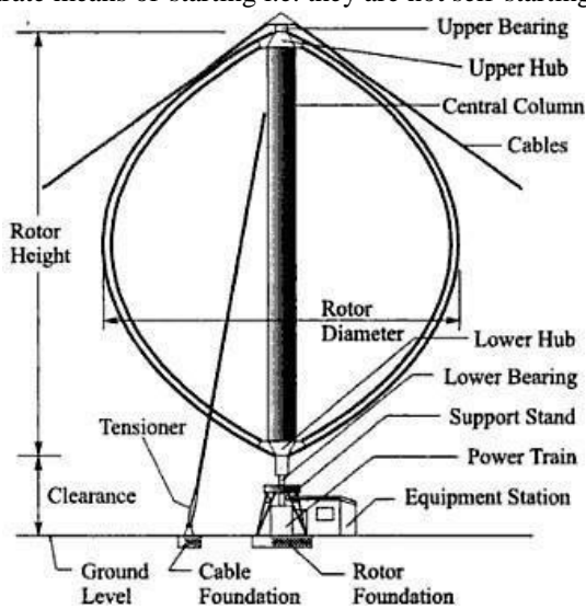
Fig.2 Vertical Axis Wind Turbine
