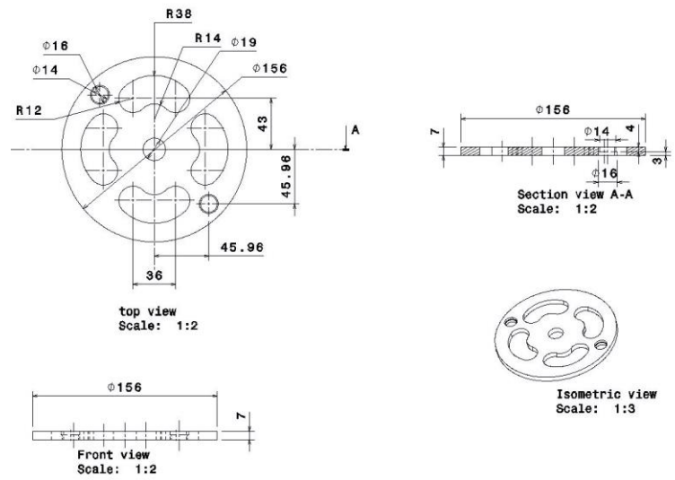
E- DISC PLATE-
