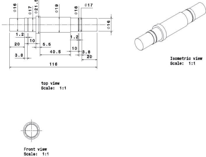
C- MAIN SHAFT-
