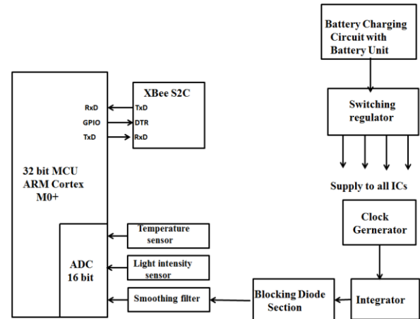
Fig. 1. Sensor node of individual plant(transmitter unit).
