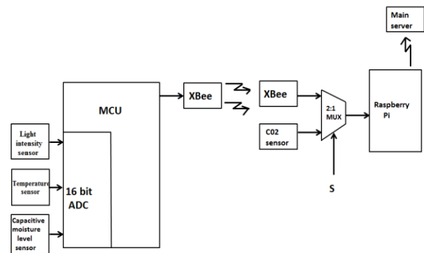
Fig. 5. Overall block diagram of the proposed system.
