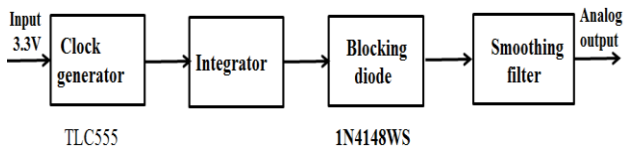
Fig. 3. Block diagram of capacitive type moisture level sensor.
