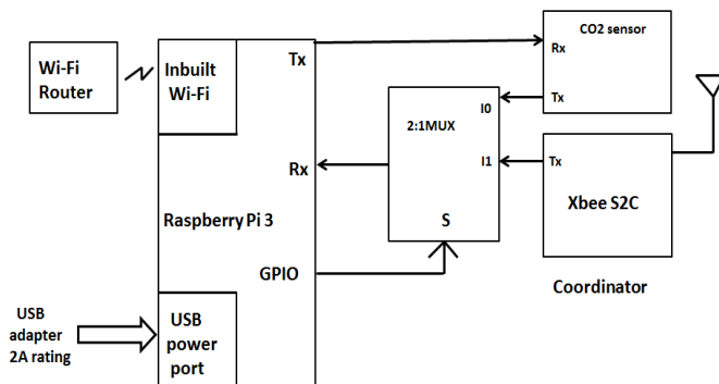
Fig. 4. The brain unit (receiver unit).
