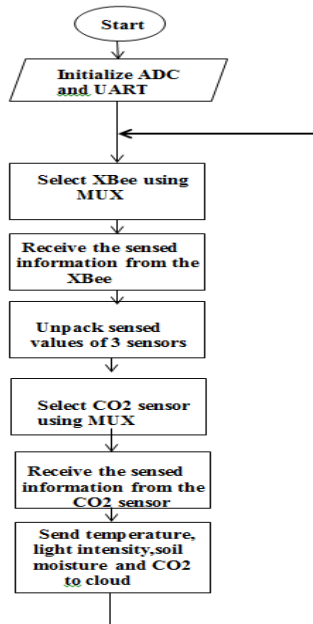
Fig. 8. Overall program flow of the receiver part.
