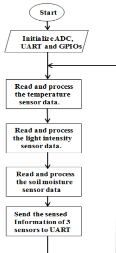
Fig. 7. Overall program flow of the sensor node part.
