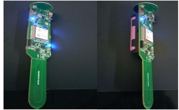
Fig. 9. Hardware module of sensor node.
