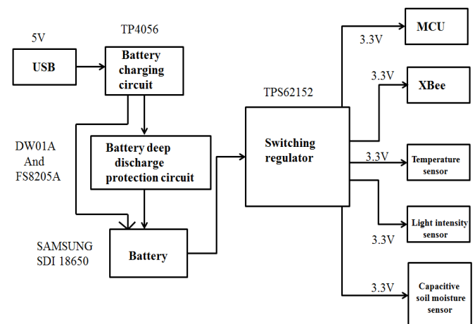
Fig. 2. Battery charging part and switching regulator part.
