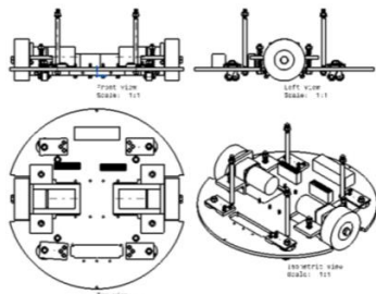
Fig. 3. Robot Assembly
