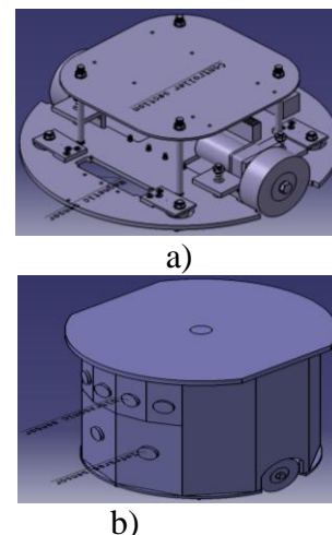
Fig.1. (a) 3D model of the chassis (b) Whole body of the robot platform
