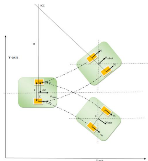
Fig.5. The Robot Motion model
