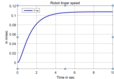
Fig.13. Simulink result of motor speed with K_p=1 , K_I=0 and K_D=0
