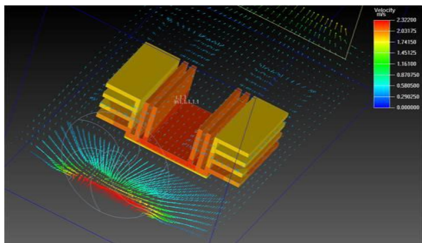
Fig. 6. Thermal image of Heat sink for Fan on side condition at 25 W
