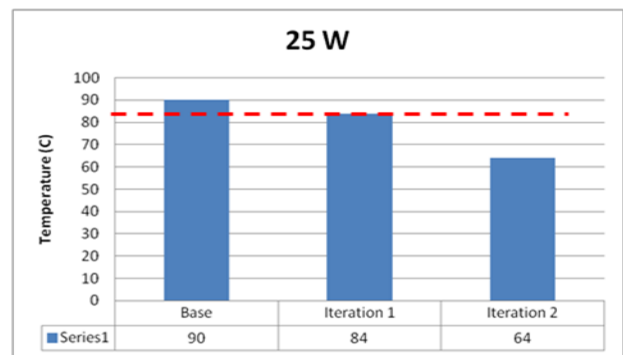
Fig. 18. Graph of Comparison of Case-I and Case-II at 25 W
