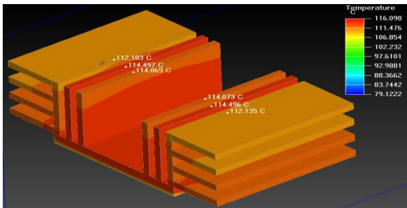
Fig. 12. Thermal image of Heat sink for Fan Failed condition at 65 W
