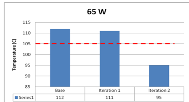
Fig. 19. Graph of Comparison of Case-I and Case-II at 65 W
