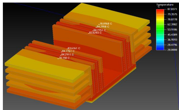
Fig. 13. Thermal image of Heat sink (Case-I) for Fan Failed condition at 25 W
