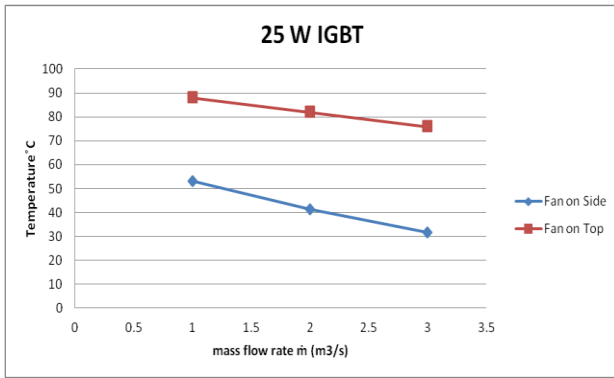
Fig. 3. Temp. Vs mass flow rate at 25 W
