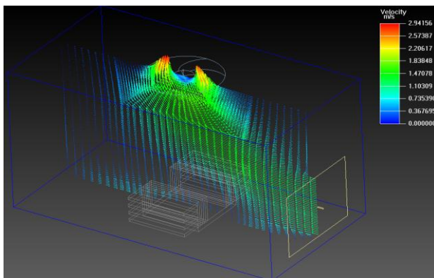
For Fan on Top condition and at 25 W (IGBT)
