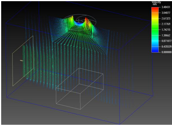
Fig. 11. Velocity vector image of Heat sink for Fan on side condition at 65W
