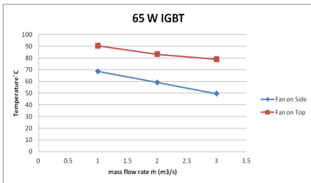
Fig. 4. Temp. Vs mass flow rate at 65 W
