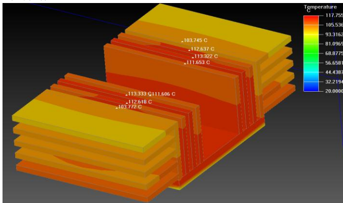
Fig. 14. Thermal image of Heat sink (Case-I) for Fan Failed condition at 65 W
