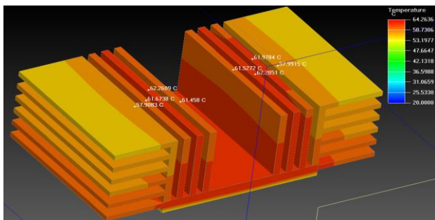
Fig. 15. Thermal image of Heat sink (Case-II) for Fan Failed condition at 25 W
