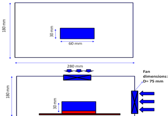
Fig. 1. Front view of experimental set up
