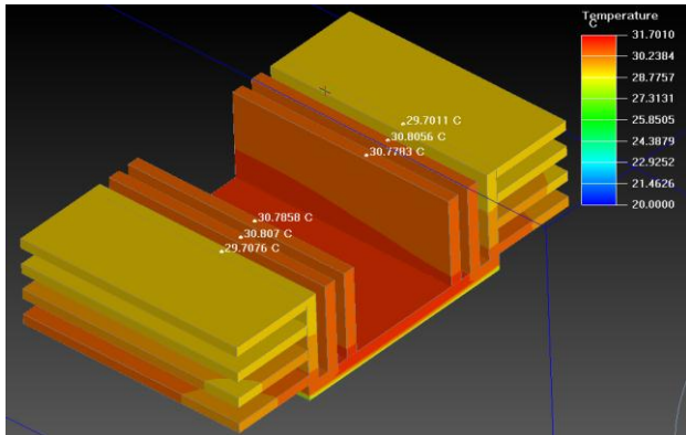
Fig. 5. Thermal image of Heat sink for Fan on side condition at 25 W
