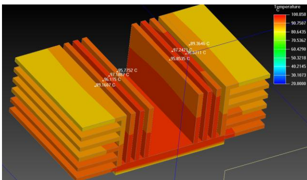
Fig. 17. Thermal image of Heat sink (Case-II) for Fan Failed condition at 65 W
