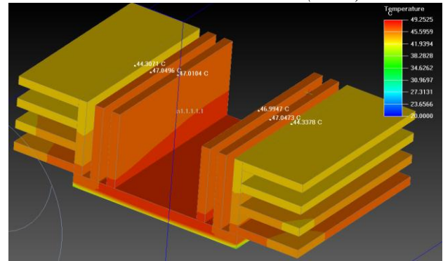
Fig. 8. Thermal image of Heat sink for Fan on side condition at 65 W
