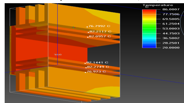
Fig. 10. Thermal image of Heat sink for Fan on Top condition at 65 W
