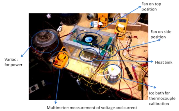
Fig.2.experimental set up
