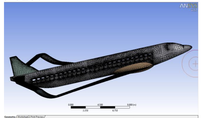
FIGURE 10 Shows the meshing at all the sections of aircraft.
