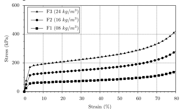
Fig. 4. Unconfined uniaxial stress strain behavior of model geofoam
