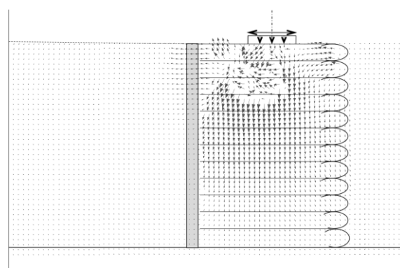
(b) With geofoam, footing at 0.5L r
