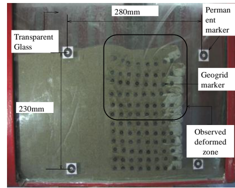
(a) Without geofoam, footing at 0.5L r
