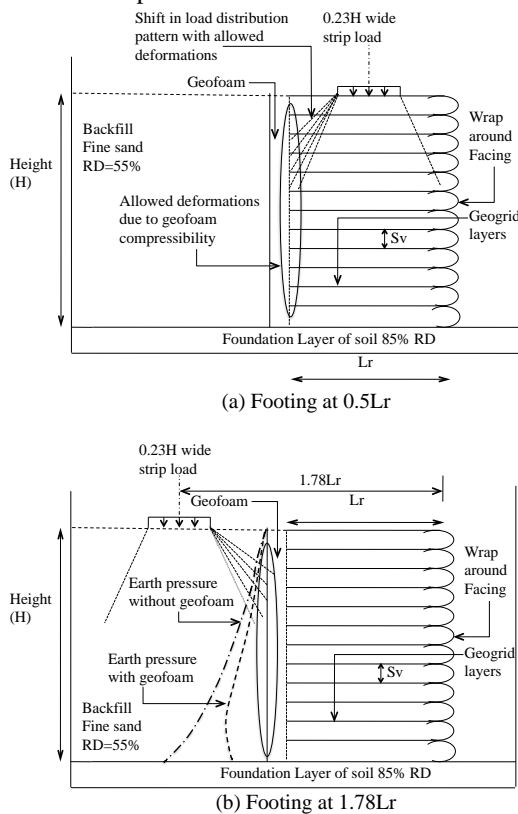
Fig. 1. Schematic cross section of geogrid reinforced soil wall with geofoam inclusion
