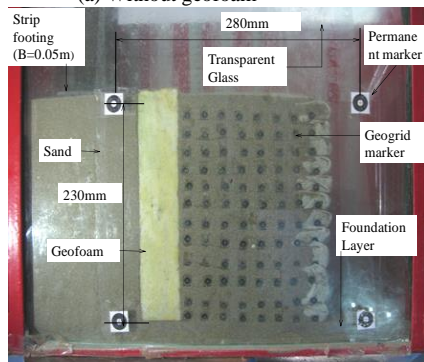
(b) With geofoam
