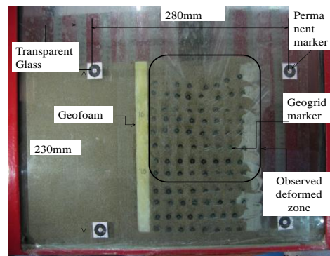
(a) With geofoam, footing at 0.5L r
