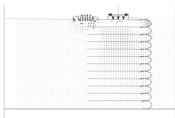
(a) Without geofoam, footing at 0.5L r
