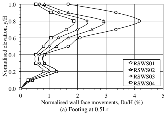
(a) Footing at 0.5Lr
