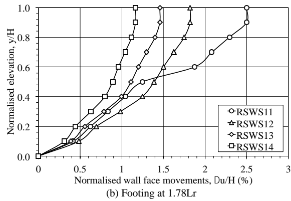
(b) Footing at 1.78Lr Fig. 8. Variation of wall face movements along the height of geogrid reinforced soil walls
