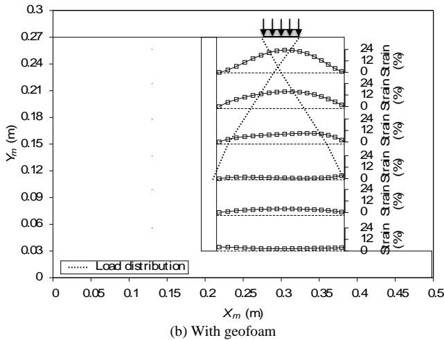
Fig. 9. Variation of wall face movements along the height of geogrid reinforced soil walls
