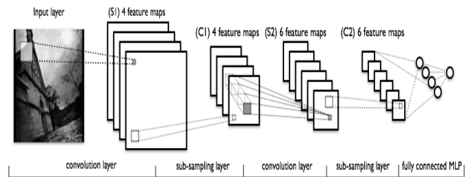
Fig. 3. Working process of CNN
