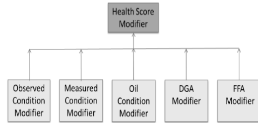
Fig.4 Health Score modifier schematic diagram
