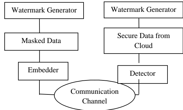
Fig 7: Watermarking Technique
