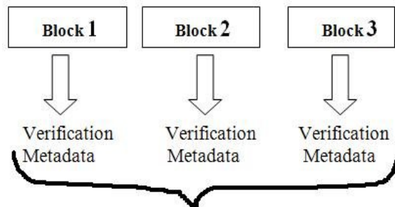
Fig 5: Homomorphic Authenticator
