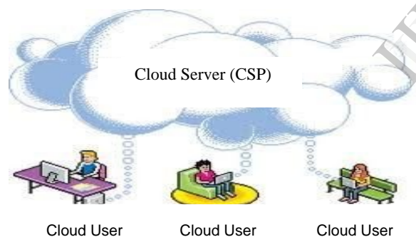
Fig 1: Cloud Architecture
