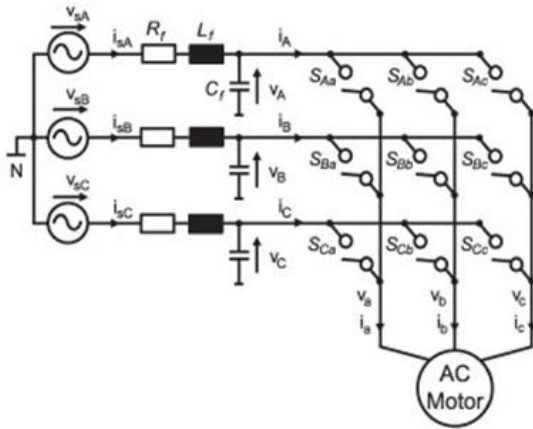
Fig.1 DMC Topology
