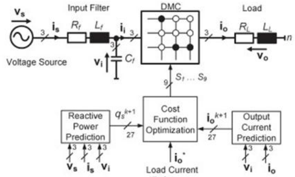
Fig .4 PCC scheme
