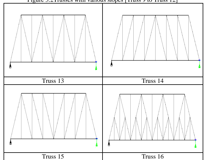
Figure 3.3 Trusses with slope and horizontal top chords [Truss 13 to Truss 16]
