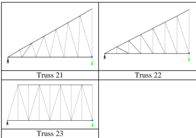
Figure 3.5 Nonsymmetrical trusses [Truss 21 to Truss 23]
