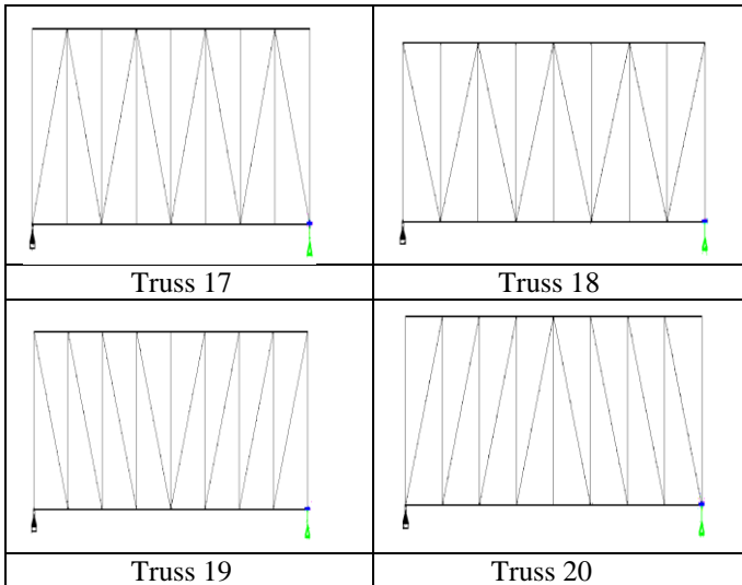
Figure 3.4 Trusses with horizontal top chords [Truss 17 to Truss 20]
