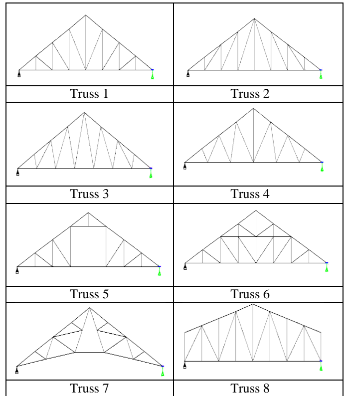
Figure 3.1 Trusses with constant slopes [Truss 1 to Truss 8]
