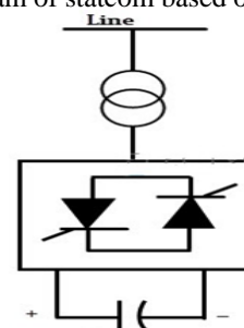
Fig.6 STATCOM structure
