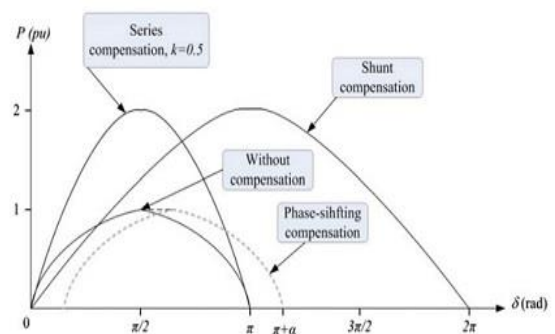
Fig.3 P-δ curve
