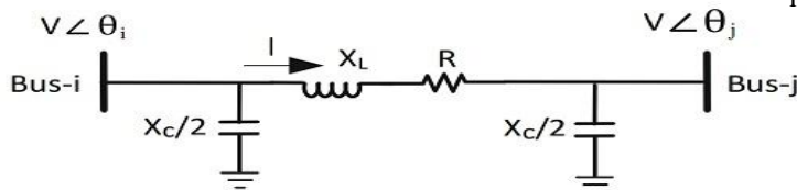
Fig.1 π-model single line diagram
