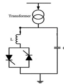
Fig.4 SVC building block
