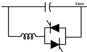
Fig.8 TCSC structure
