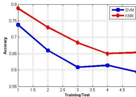
Fig. 5.1 Accuracy graph
