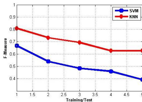
Fig. 5.2 F-measure graph
