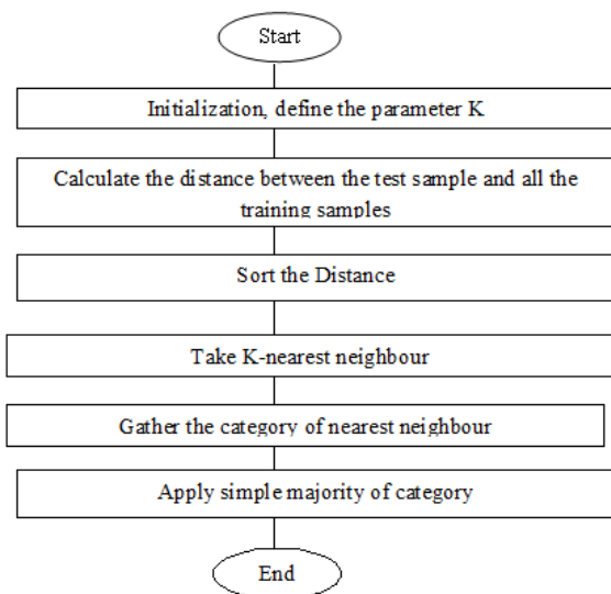
Fig. 4.1. K-NN working
