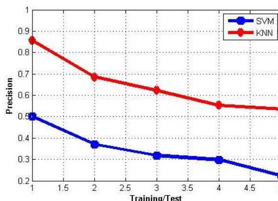
Fig. 5.3 Precision graph
