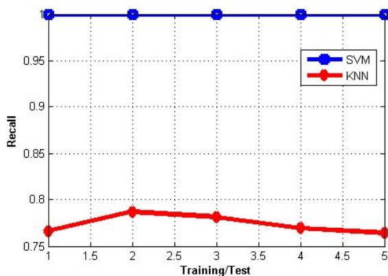
Fig. 5.4 Recall graph
