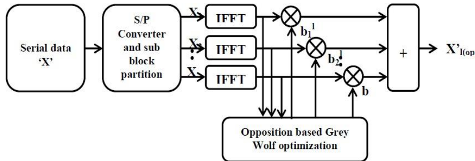
Figure 1. Block diagram of PTS
