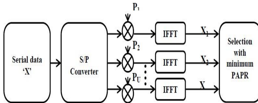
Figure 2: Block diagram of SLM
