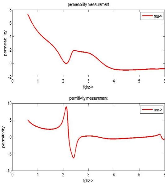
Fig 2(b) CSRR Permeability and permittivity curve with respect to frequency.
