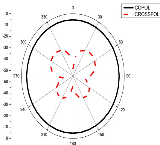
Fig 3(c) H-plane at \phi=0^\circ
