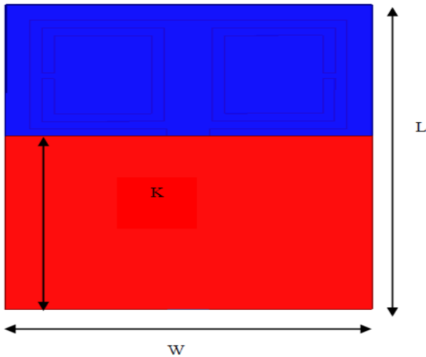
Fig 3(b) Bottom view of the proposed antenna
