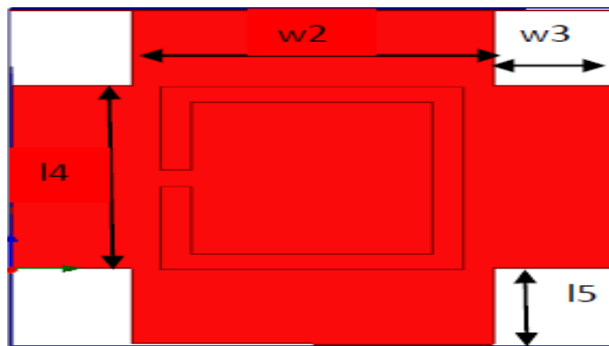
Fig 1 (b) CSRR bottom view
