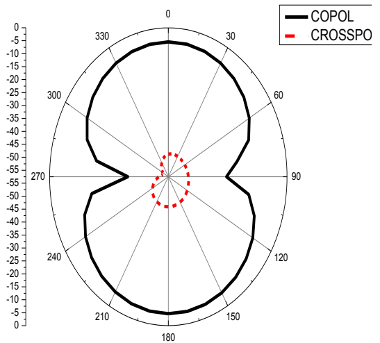
Fig 3(d) E-plane at \phi=90^\circ
