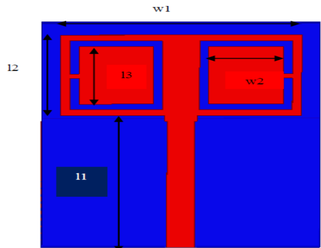
Fig 3(a) Top view of the proposed antenna
