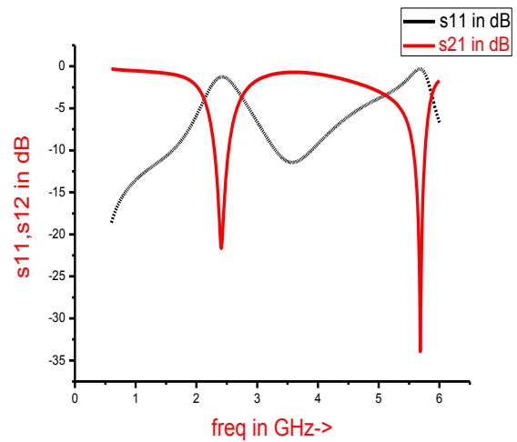
Fig 2(a) Reflection and transmission coefficient vs. frequency.
