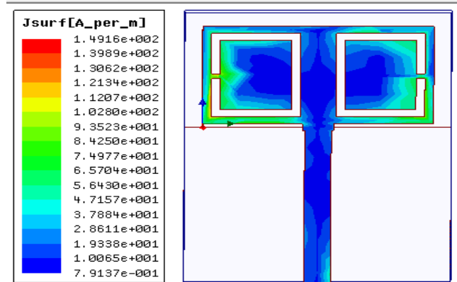
Fig 3(e) Magnitude of surface current density( J_{surf} in A/m)
