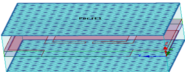
Fig 1 (d) PEC boundary applied at z=-5.035, 6.635 plane & PMC in ZX plane.
