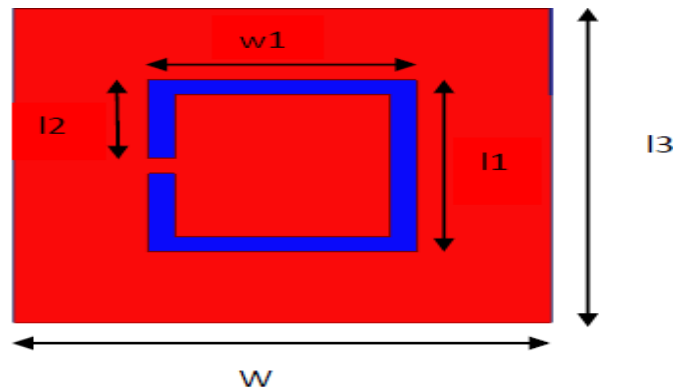
Fig 1 (a) CSRR top view
