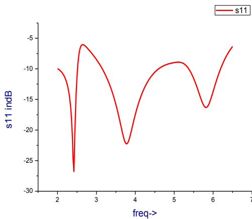
Fig 3(b) Return loss vs. frequency curve
