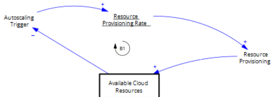
Figure 2. Causal loop 1
