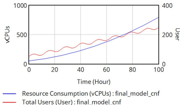
Figure 7: Resource Consumption and Total Users
