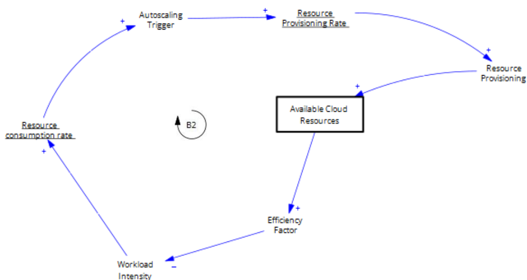
Figure 3. Causal loop 1
