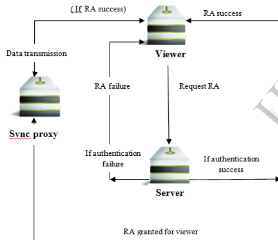
Fig1.VNC based architecture
