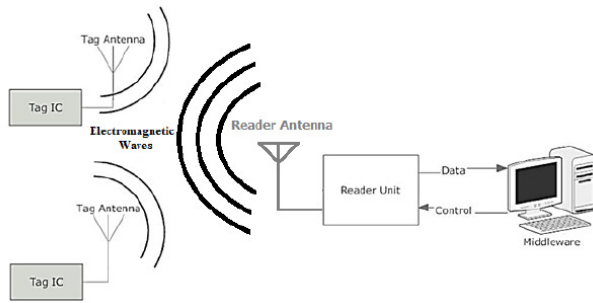
Figure 1. Components of RFID system
