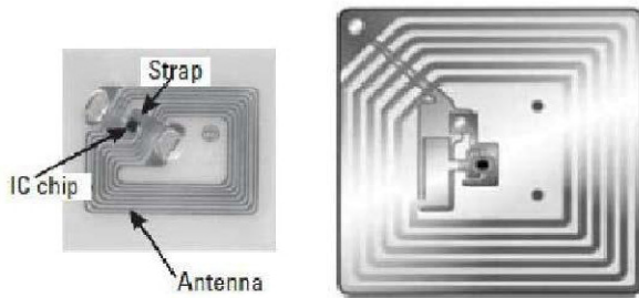
Figure 2. Typical design of passive tag
