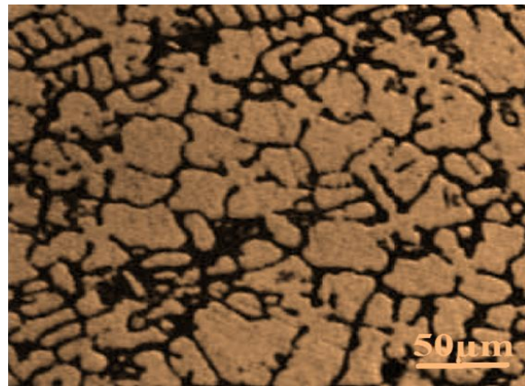
Figure1. Optical photomicrographs: unreinforced A357 alloy reinforced with 1.5 vol. % SiC.
