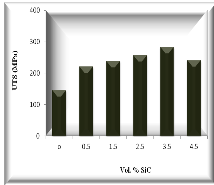
Figure9. Variations of UTS as a function of vol. % nano-SiC particulates
