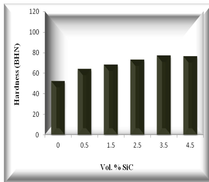
Figure 6. Variation of hardness as a function of vol.% SiC particulates
