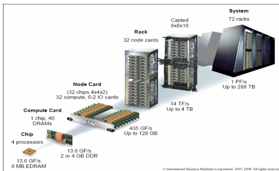
Figure 4: Blue brain Storage hierarchy
