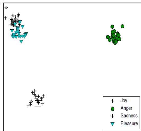
Figure 4: 2D Fisher projection (4 classes)
