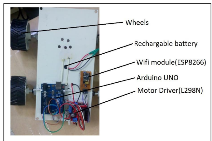
Fig. 3. Circutary of Lawn Mower
