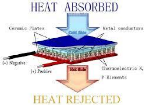
FIG 1: OVERVIEW OF PELTIER DEVICE
