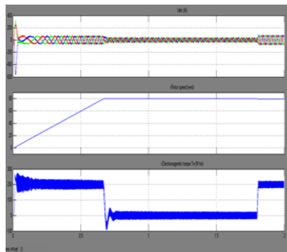
Fig 5.13 Result for variable torque and constant Speed condition
