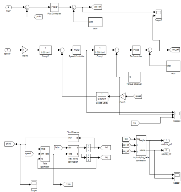
Fig 5.4 Vector Control
