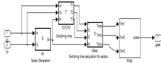
Fig 5.5 Pulse Generation
