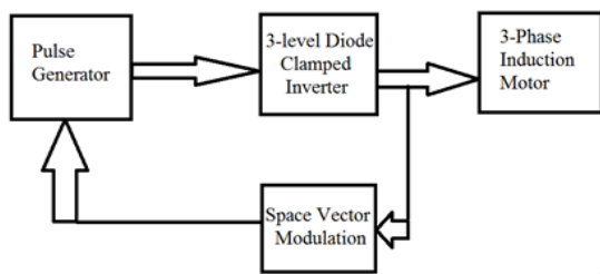
Fig. 5.1 Block Diagram of induction motor fed by NPC inverter
