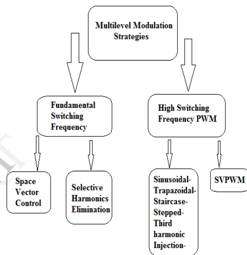
Fig. 3.1 Overviews of different modulation strategies
