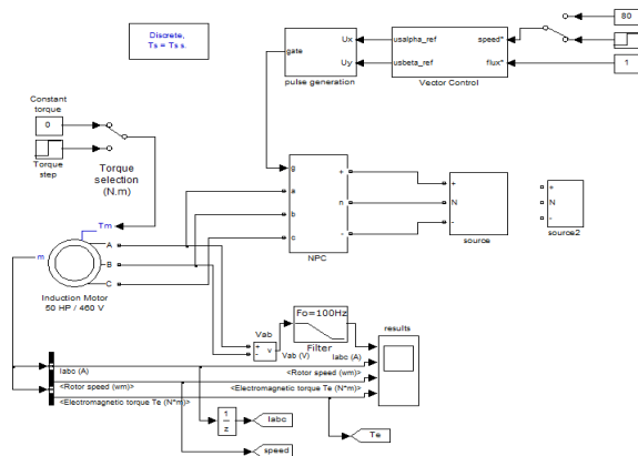
Fig. 5.1 Simulation of Main model
