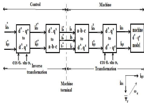
Fig 2.8 Vector control implementation principle
