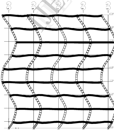
Figure 4.12 Mode 12 period 0.1522 sec frequency 7.320
