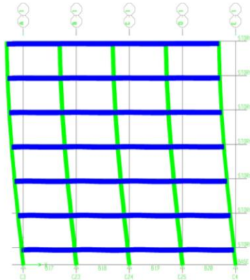
Figure 4.7 Mode 1 period 1.0526 sec frequency 0.950
