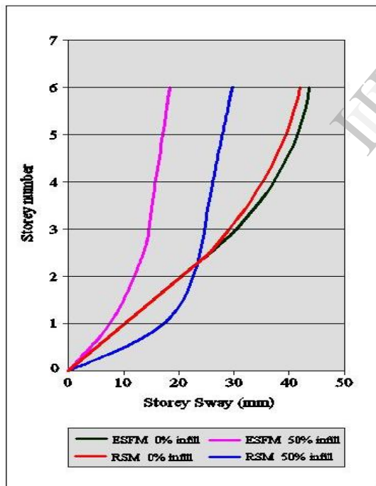
Fig.4.14 Storey sway for 6 storied Building for 50% infill and for No infill condition
