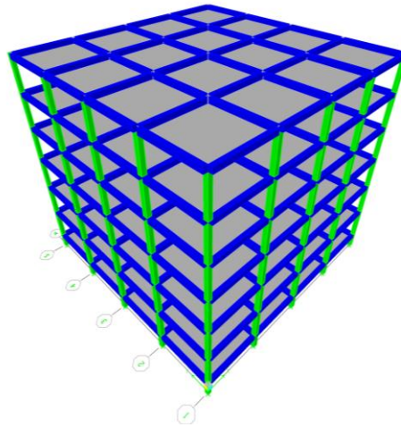
Figure 3.1 Structural model
