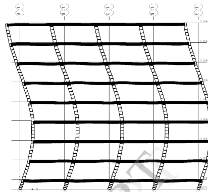
Figure 4.11 Mode 5 period 0.4217 sec frequency 2.056
