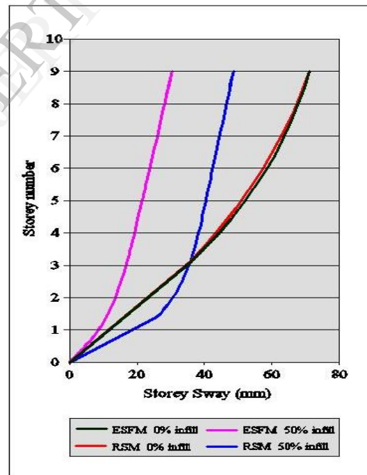
Fig 4.15 Storey sway for 9 storied Building for 50% infill and for No infill condition
