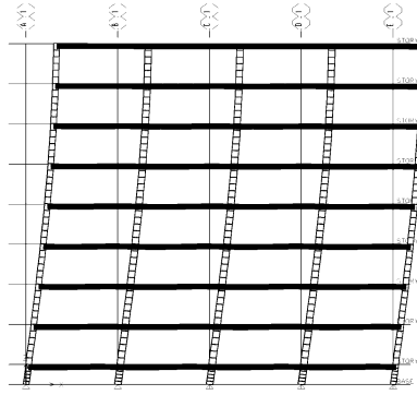
Figure 4.10 Mode 1 period 1.3089 sec frequency 0.8674
