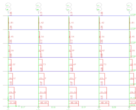
Figure 4.6 Distribution of axial force in column due to response spectrum earthquake load for 50 percent infill condition
