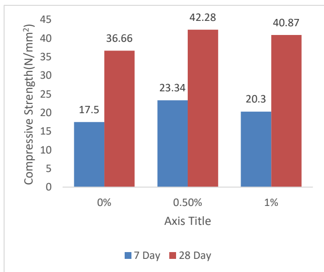
Fig : Compressive strength of concrete with 10% marble powder and different % water hyacinth
