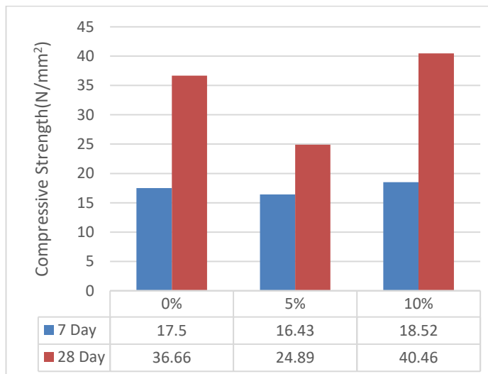
Fig Compressive strength pf concrete with various percentage of marble powder.
