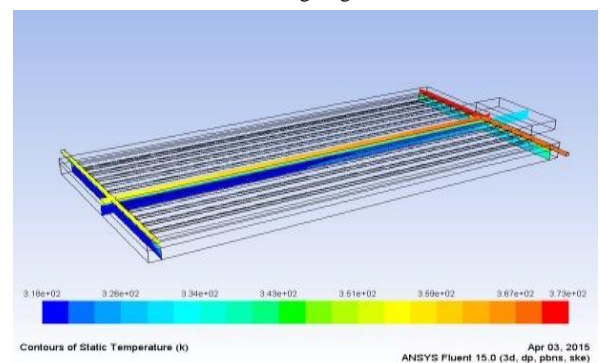
Fig 4.4.1(A) Temperature Distribution for DPSC with Circular Profile with Zig-Zag Path
