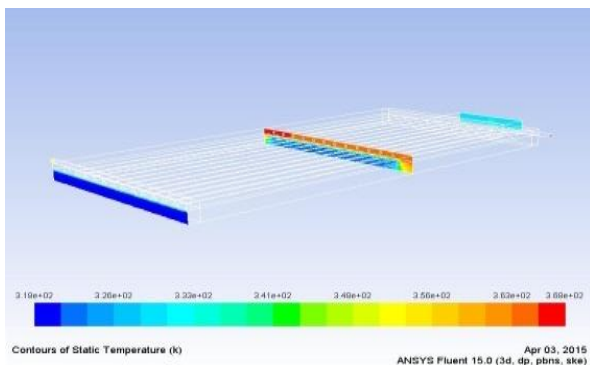
Fig 4.3.1(A) Temperature Distribution for DPSC with Circular Profile
