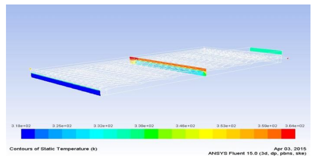
Fig 4.4.1(A) Temperature Distribution for DPSC with Circular Profile with Zig-Zag Path
