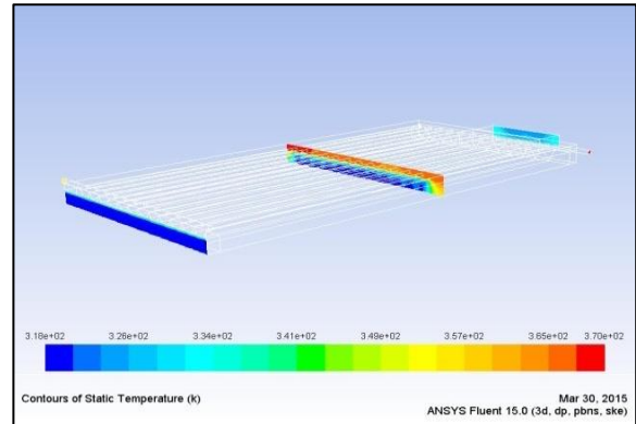
Fig 4.1.1 Temperature Distribution for DPSC with Triangle Profile (Base Case)
