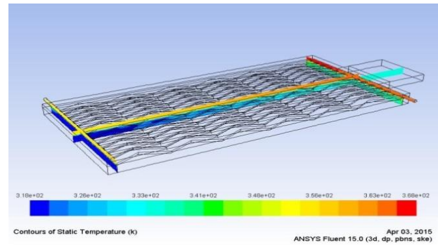
Fig 4.3.1(B) Temperature Distribution for DPSC with Circular Profile
