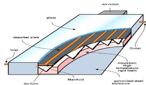
fig 1.1(B) Dual Purpose Solar Collector
