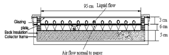
fig 1.1(A) Dual Purpose Solar Collector
