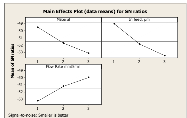
Fig. 4. Main Effects Plot (data means) for SN ratios (Signal to Noise: Smaller is better) for Boric Acid.
