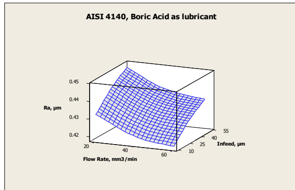
Fig. 11. AISI 4140, Boric Acid as lubricant
