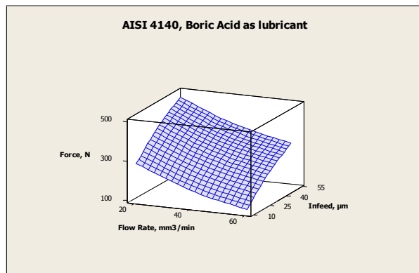
Fig. 6. AISI 4140, Boric Acid as lubricant
