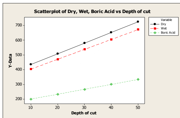
Fig. 3. Surface roughness for AISI 4140 using different coolants.
