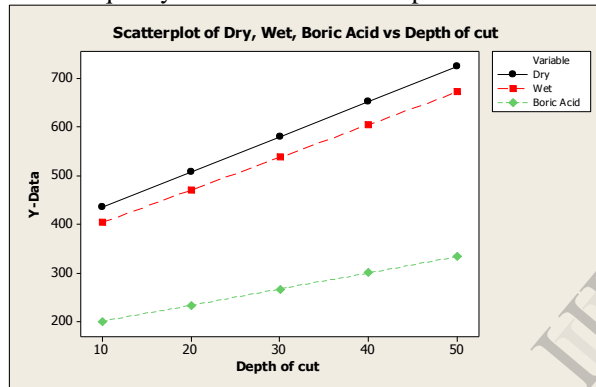
Fig. 2. Effect of coolants on force under varying depths of cut
