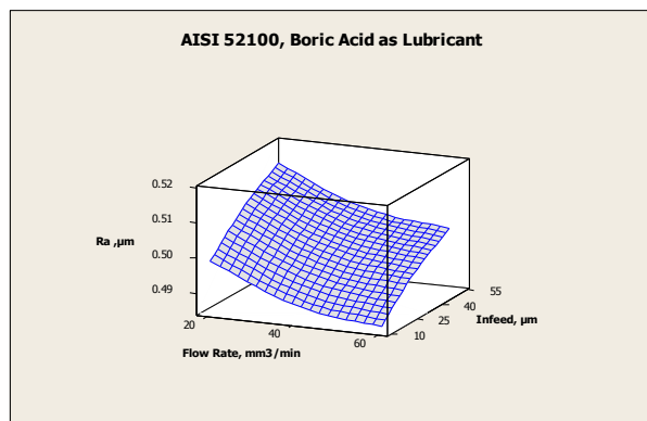
Fig. 13. AISI 52100, Boric Acid as lubricant
