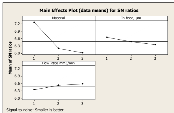
Fig. 9. Main Effects Plot (data means) for SN ratios (Signal to Noise: Smaller is better) for Boric Acid
