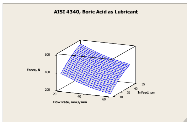
Fig. 7. AISI 4340, Boric Acid as lubricant
