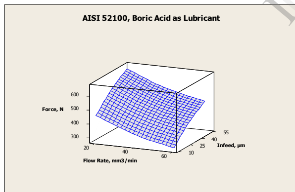
Fig. 8. AISI 52100, Boric Acid as lubricant
