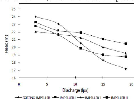
Figure 2. Head developed by the existing and modified impellers
