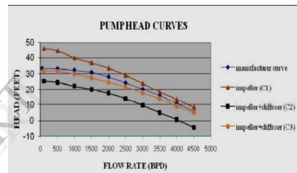
Figure 5. Results obtained in the simulations and manufacturer head curve.
