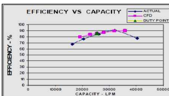
Figure 4. Efficiency versus Capacity Curve
