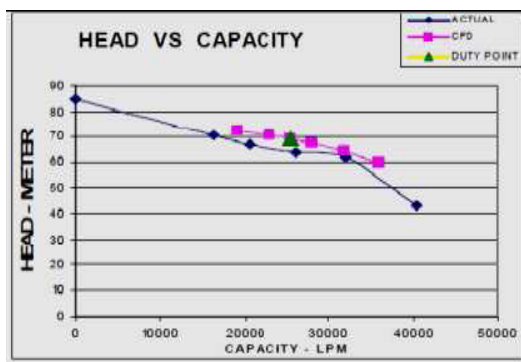
Figure 3. Head versus Capacity Curve
