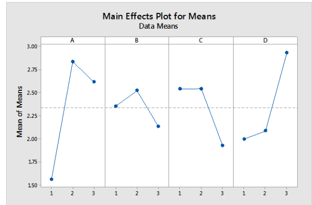
Fig.7 the main effects plot for means vs process parameters
