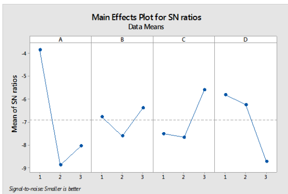
Fig.6 Mean Effect Plot Of Surface Roughness Vs Cutting Speed, Feed, Depth Of Cut And Cutting Fluid
