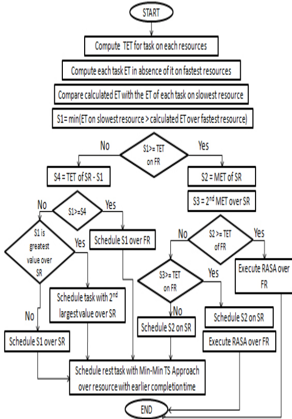
Fig 1: System Design
