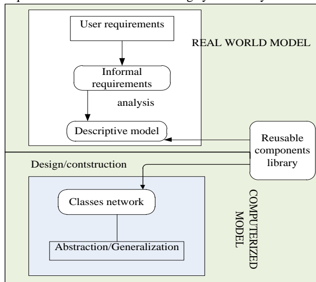
Fig. 1. Object-oriented analysis and design lifecycle [source: Nerson, 2006]
