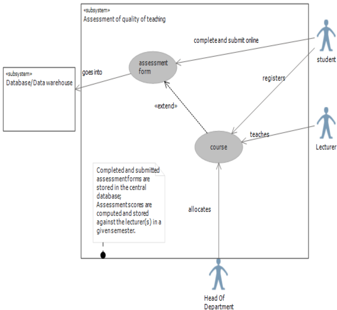
Fig. 3. Use case diagram of the proposed system
